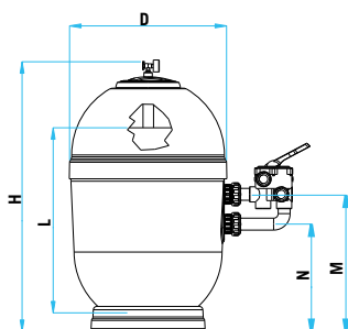
Filtro lateral Side-mount filter
