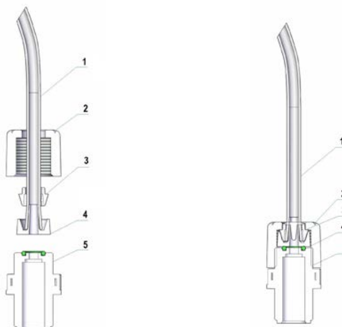
Fig.4 – Tubes connection
