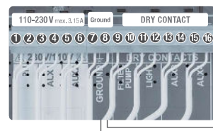
Setup and connection of a Variable Speed Pump, see section 13 - Variable Speed Pump
